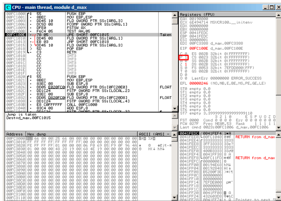
Figure 1.71: OllyDbg: TEST has been executed
