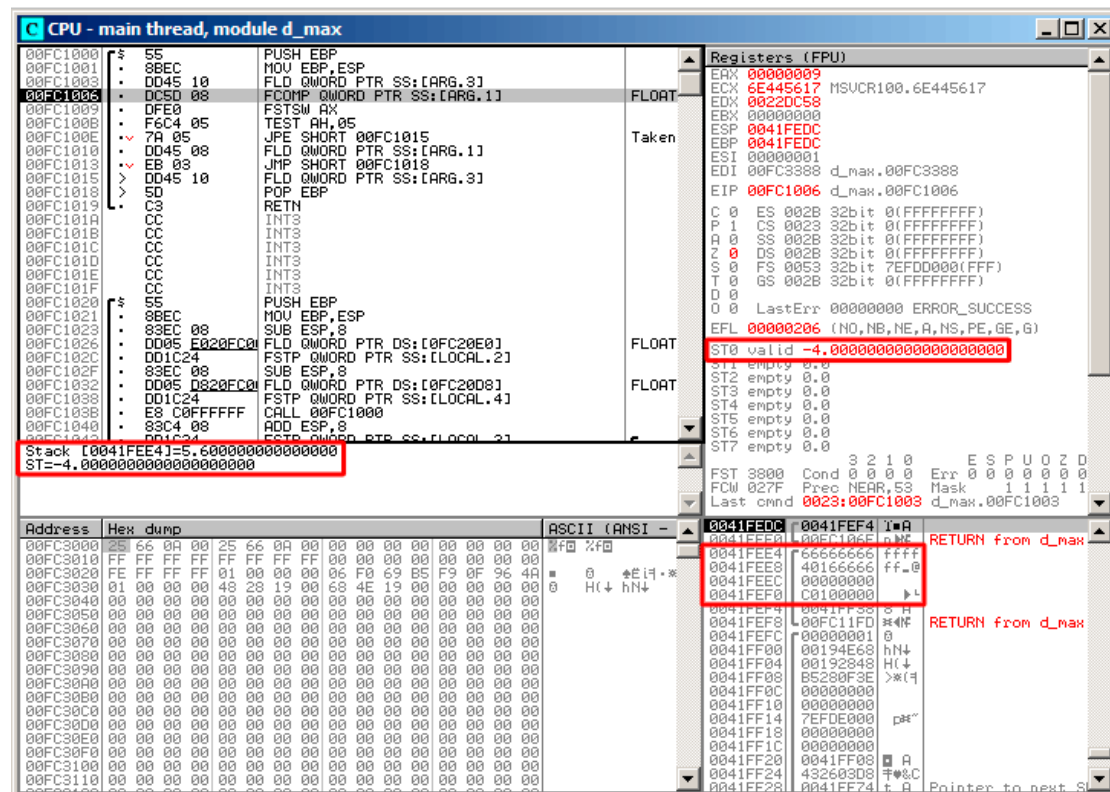
Figure 1.73: OllyDbg: first FLD executed
