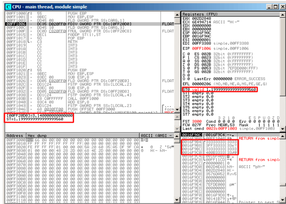
Figure 1.63: OllyDbg: the first FLD has been executed
