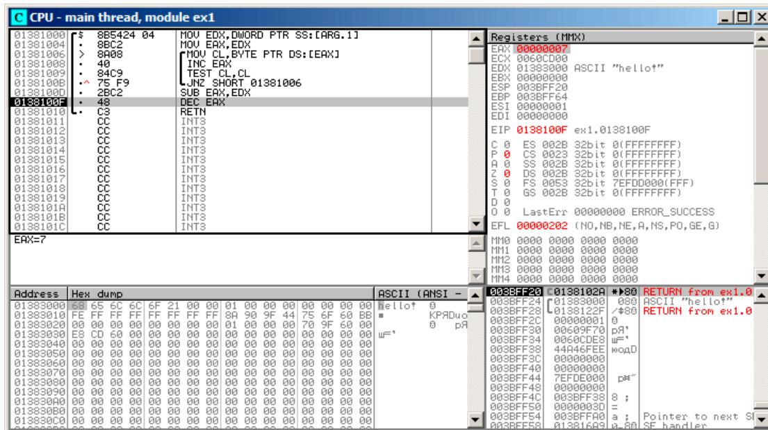
Figure 1.62: OllyDbg: EAX to be decremented now
