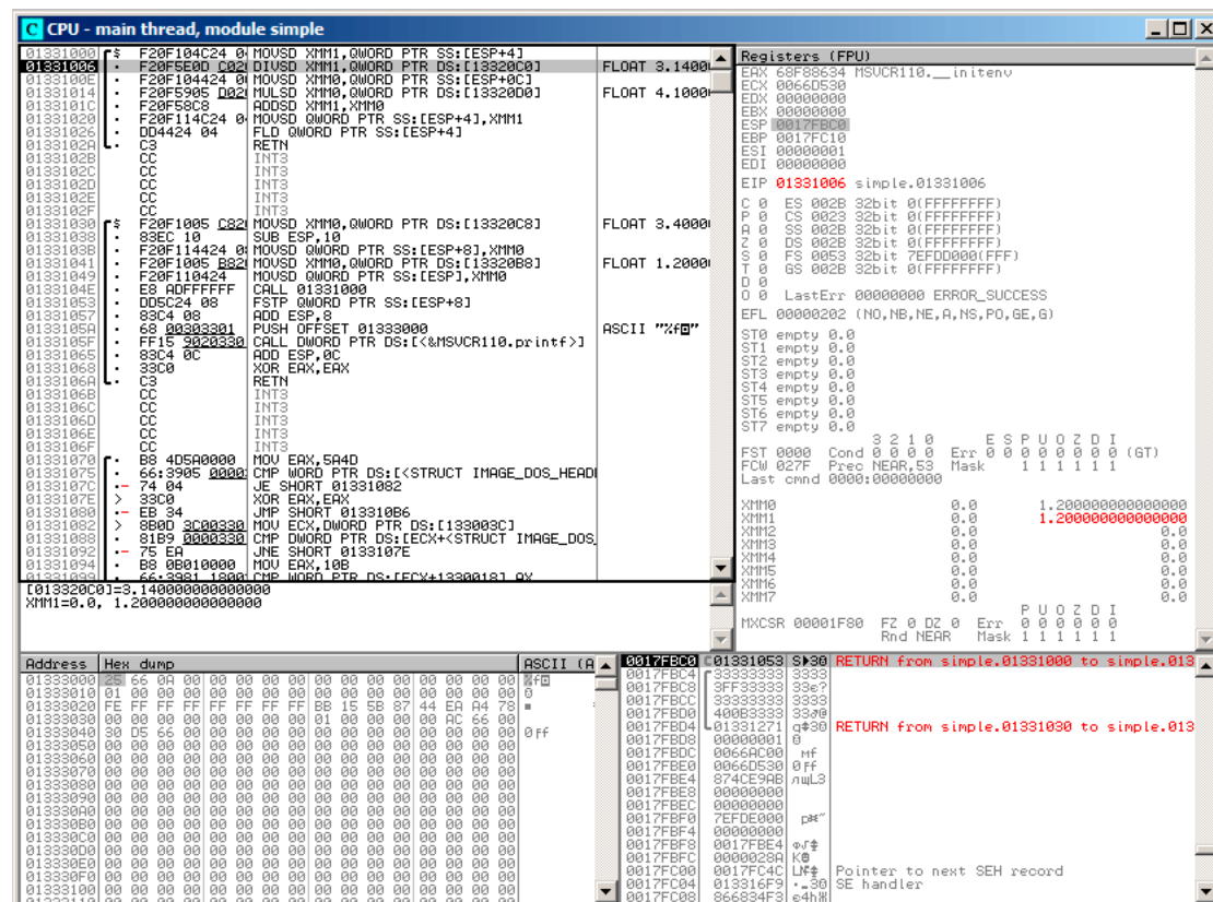
Figure 1.114: OllyDbg: MOVSD loads the value of a into XMM1
