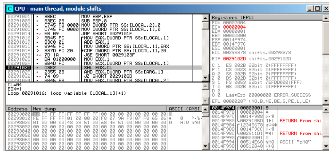
Figure 1.102: OllyDbg: i = 4 , i is loaded into ECX
