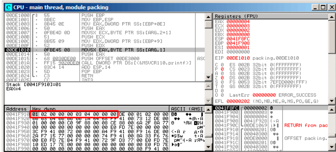
Figure 1.107: OllyDbg: Before printf() execution
