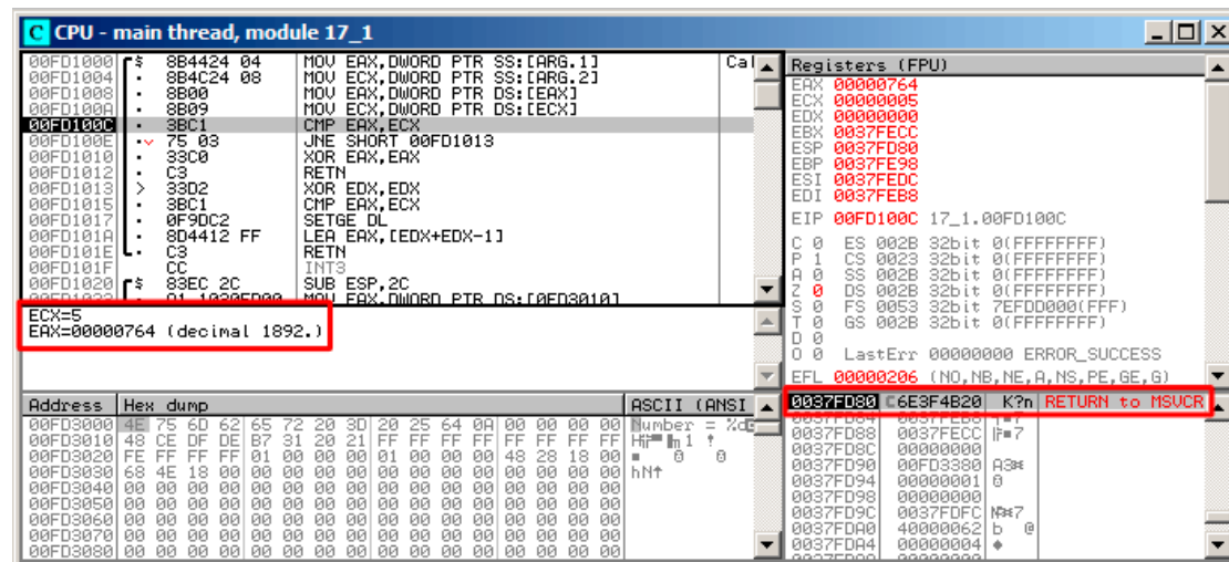
Figure 1.110: OllyDbg: first call of comp()
