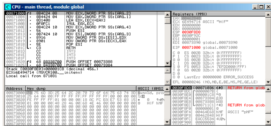
Figure 1.27: OllyDbg: f1() starts
