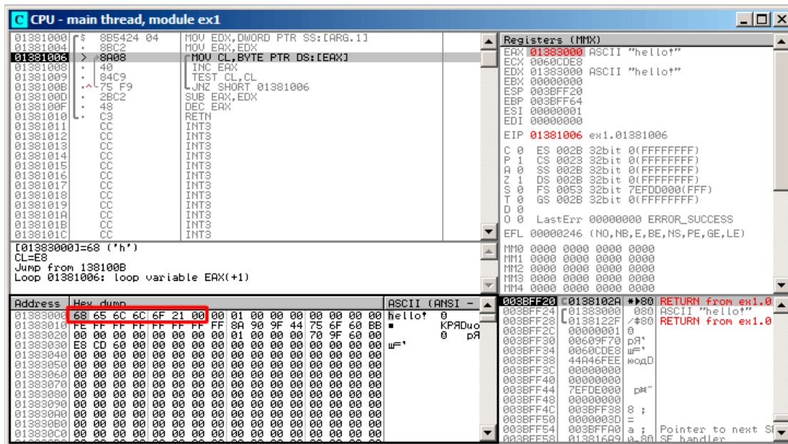
Figure 1.59: OllyDbg: first iteration start
