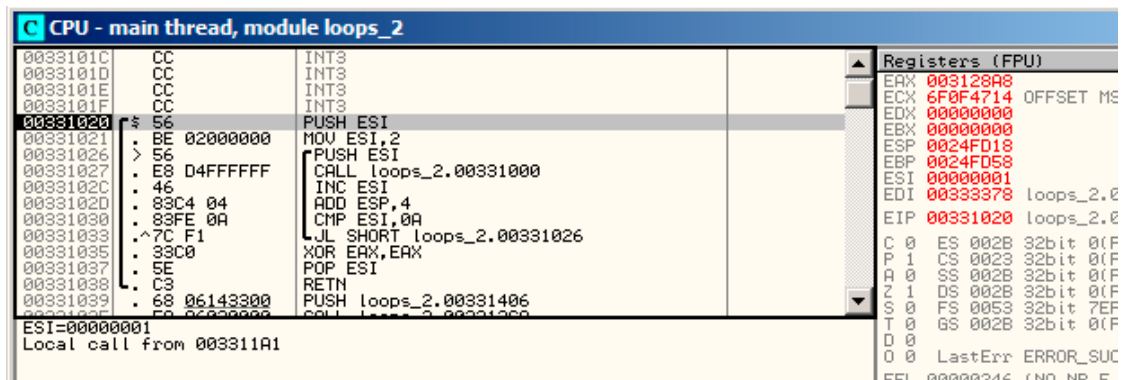
Figure 1.55: OllyDbg: main() begin
