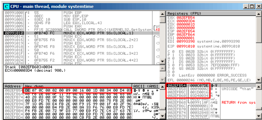
Figure 1.105: OllyDbg: GetSystemTime() just executed
