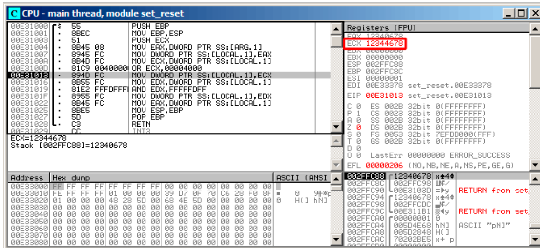
Figure 1.96: OllyDbg: 0R executed
