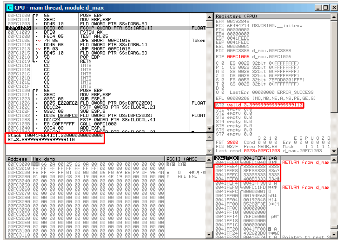
Figure 1.68: OllyDbg: first FLD has been executed
