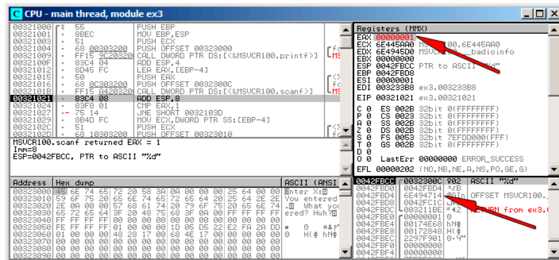
Figure 1.21: OllyDbg: scanf() returning error
