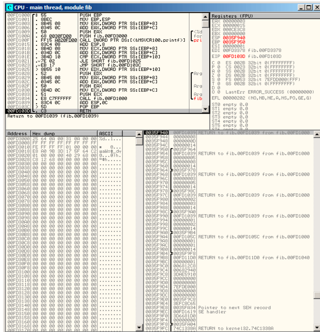
Figure 3.1: OllyDbg: last call of f()
