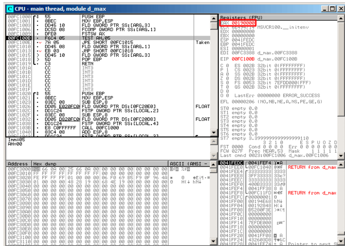
Figure 1.70: OllyDbg: FNSTSW has been executed
