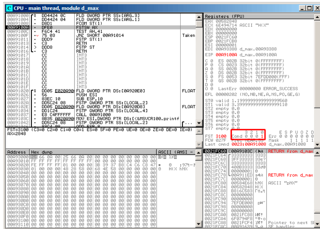
Figure 1.79: OllyDbg: FCOM has been executed
