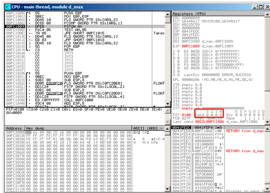
Figure 1.74: OllyDbg: FCOMP executed
