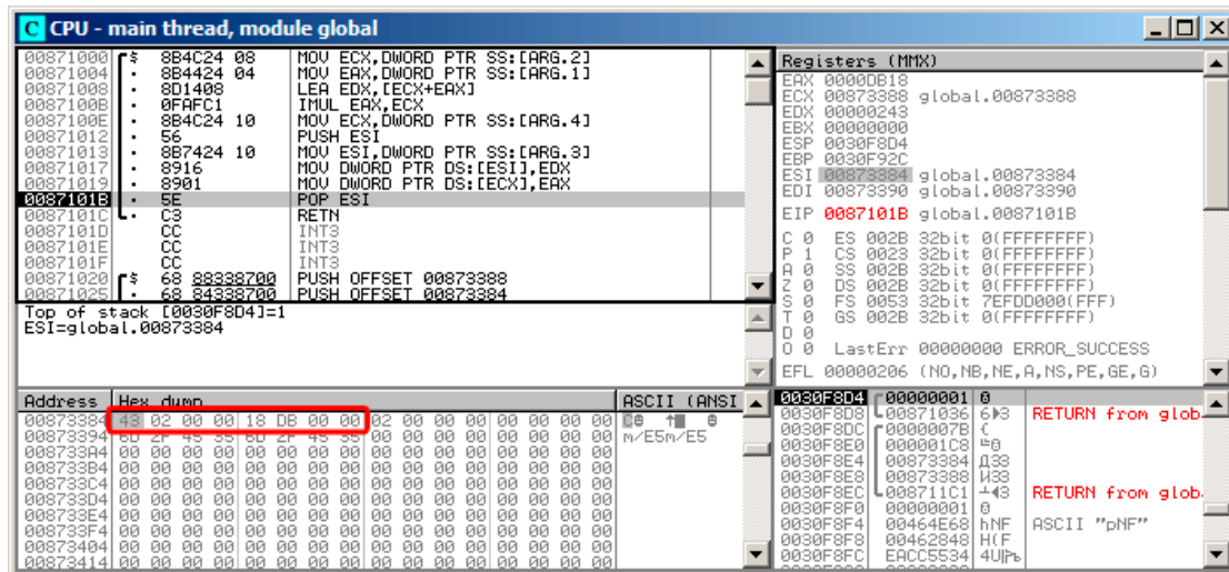
Figure 1.28: OllyDbg: f1() execution completed
