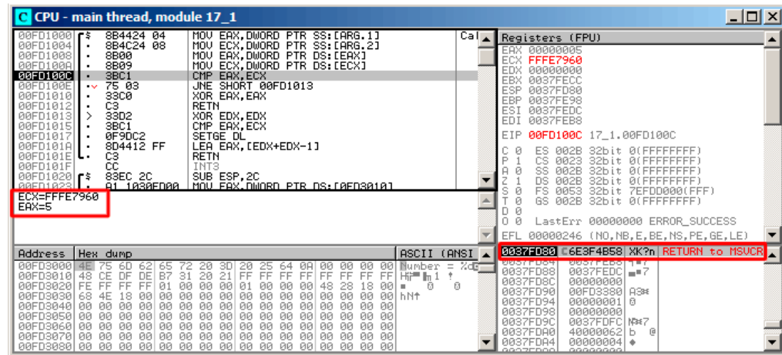
Figure 1.112: OllyDbg: second call of comp()
