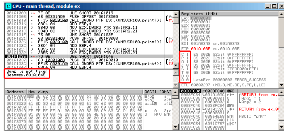
Figure 1.40: OllyDbg: f_signed(): third conditional jump
