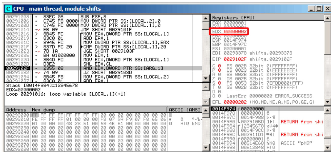
Figure 1.100: OllyDbg: i = 1 , EDX = 1 \ll 1 = 2
