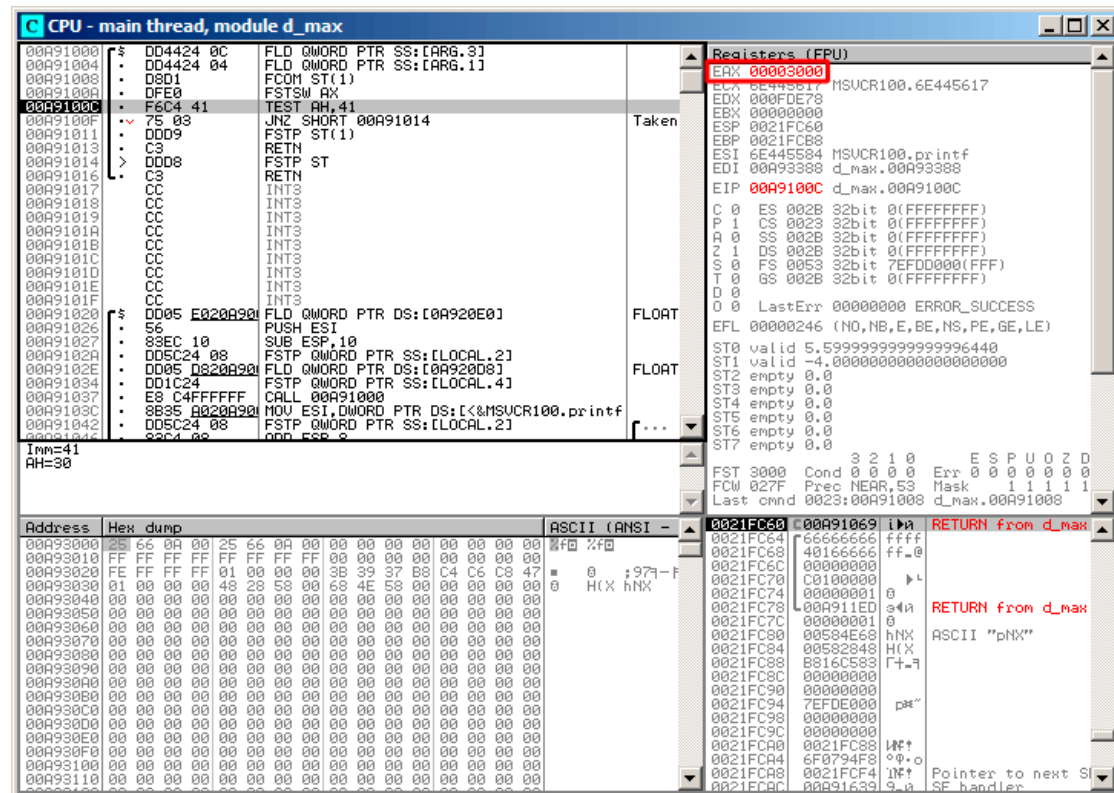
Figure 1.85: OllyDbg: FNSTSW has been executed
