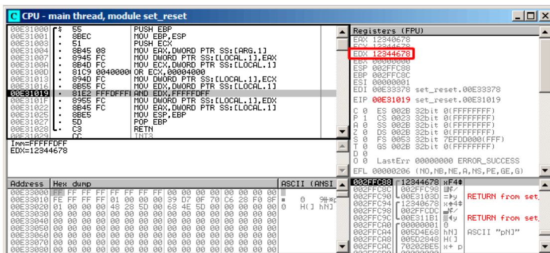
Figure 1.97: OllyDbg: value has been reloaded into EDX
