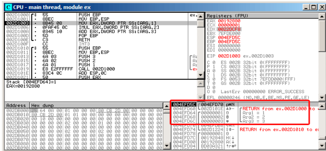
Figure 1.24: OllyDbg: inside of f() function
