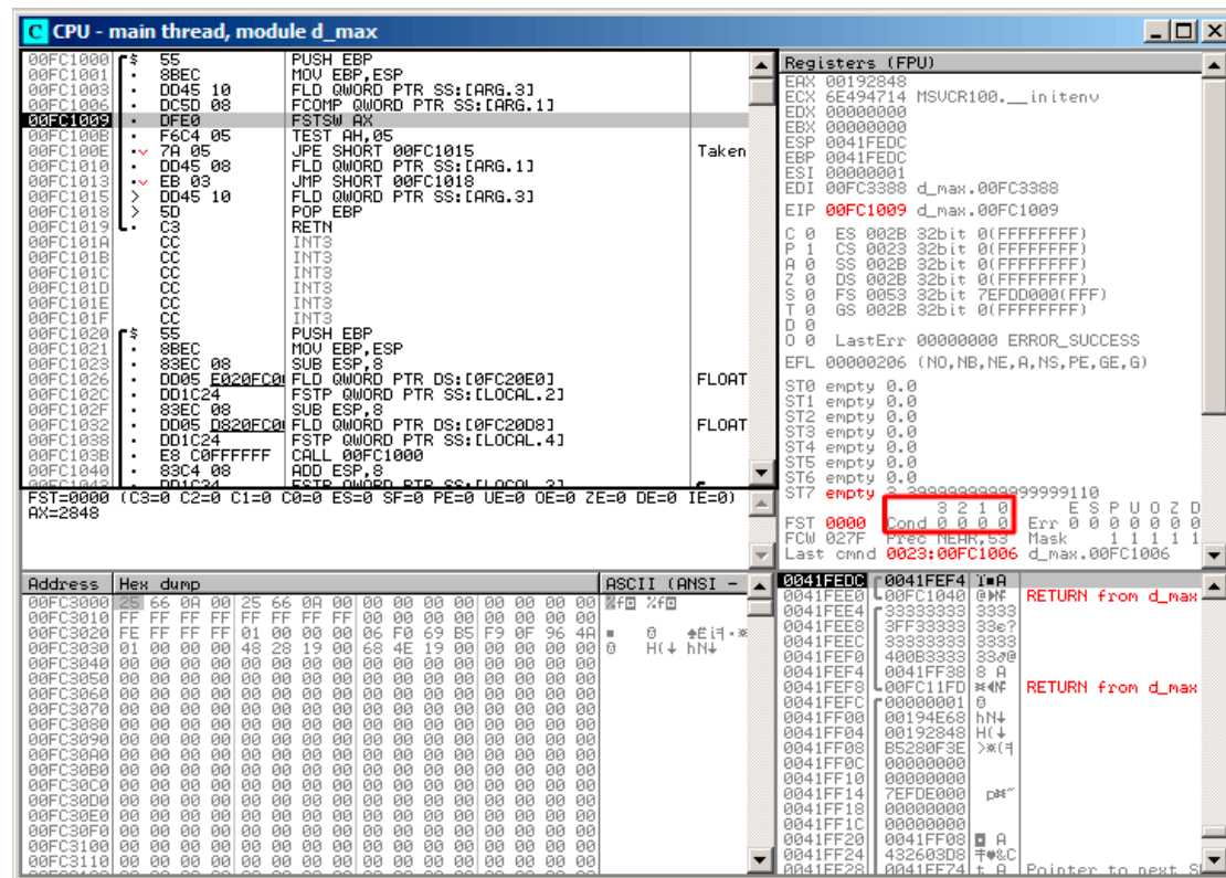
Figure 1.69: OllyDbg: FCOMP has been executed
