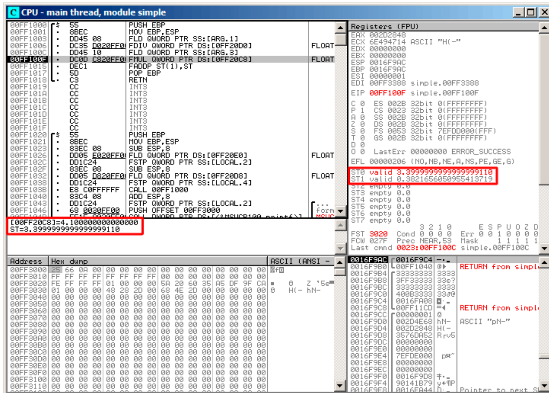
Figure 1.65: OllyDbg: the second FLD has been executed
