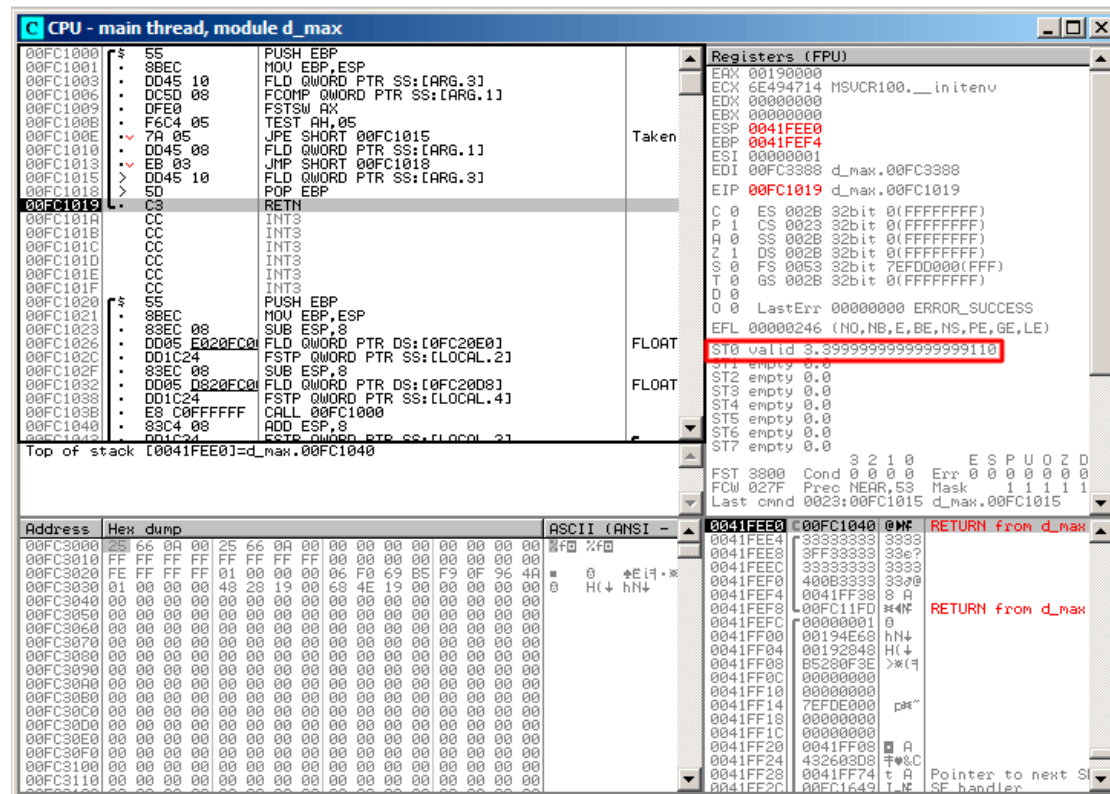
Figure 1.72: OllyDbg: the second FLD has been executed
