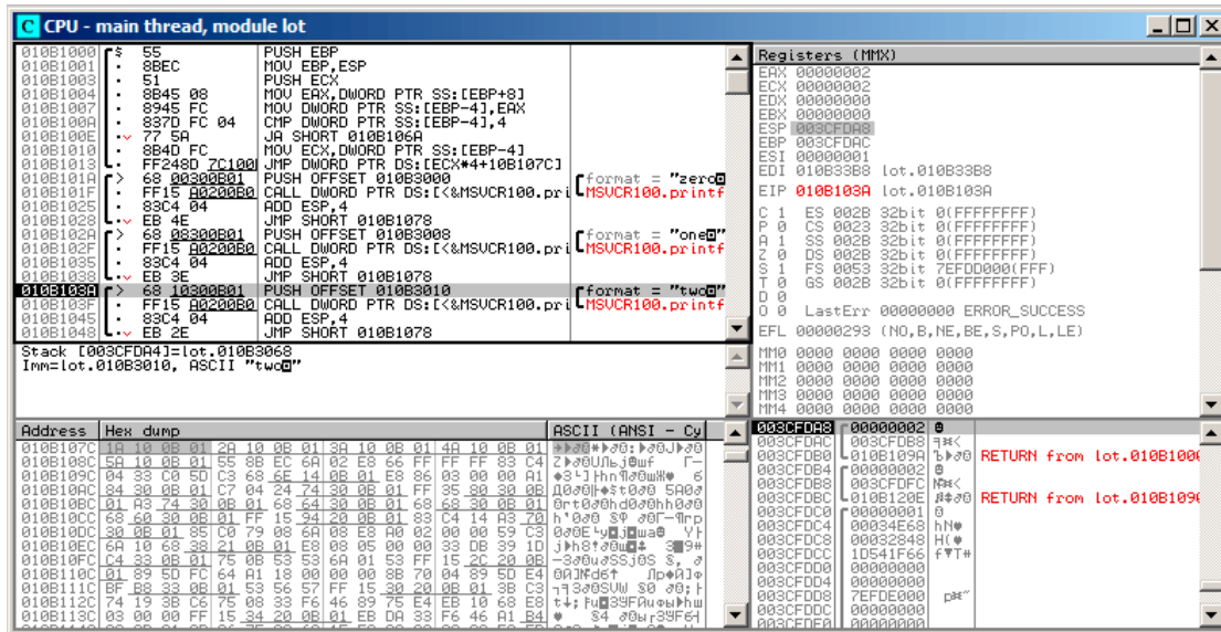
Figure 1.54: OllyDbg: now we at the case: label
