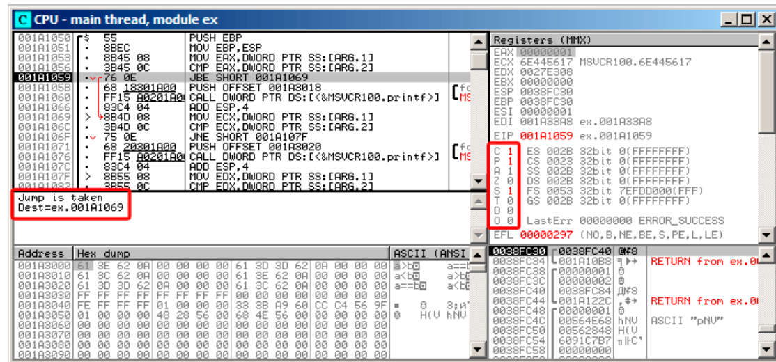
Figure 1.35: OllyDbg: f_unsigned() : first conditional jump
