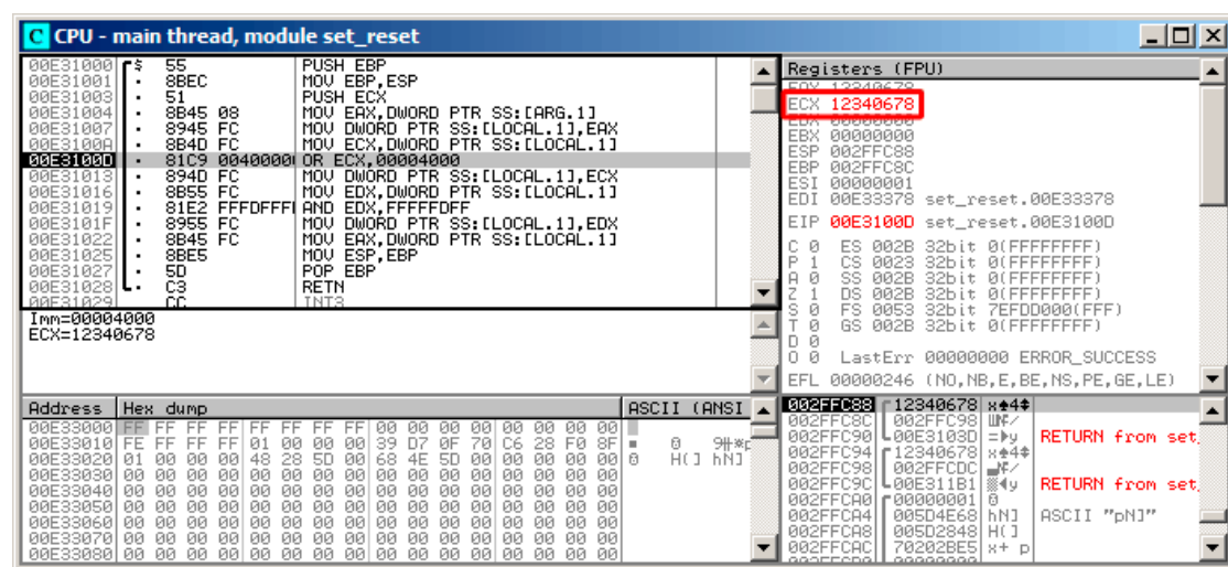
Figure 1.95: OllyDbg: value is loaded into ECX
