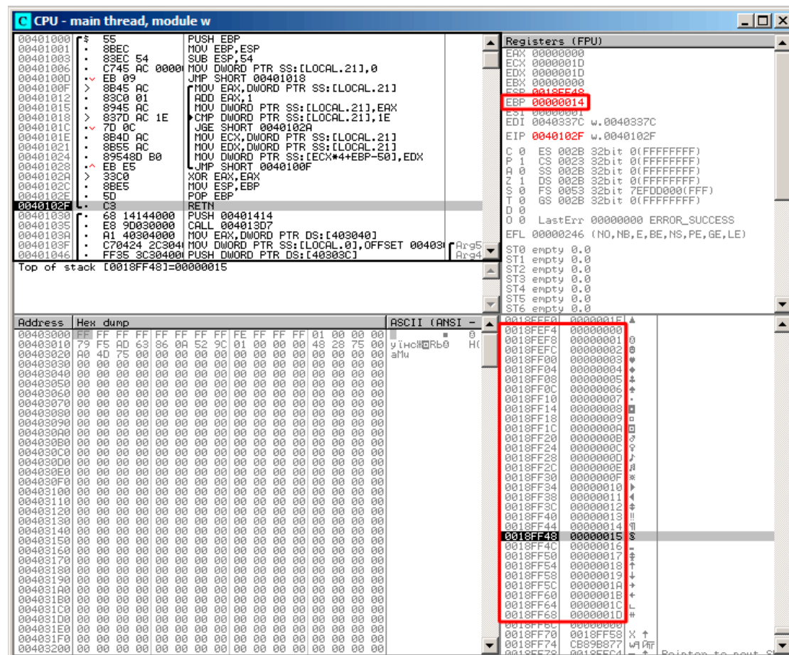
Figure 1.91: OllyDbg: after restoring the value of EBP
