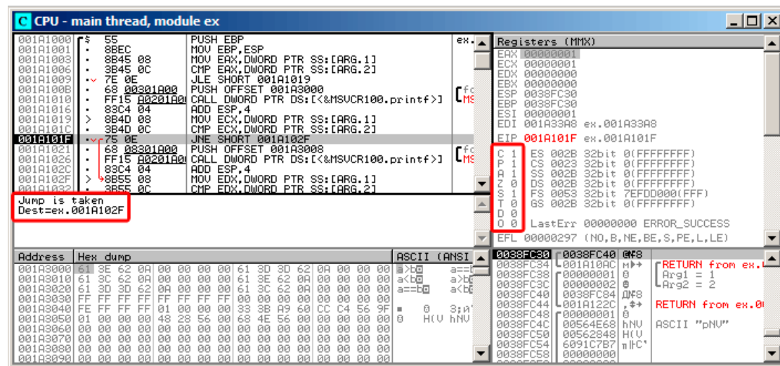
Figure 1.39: OllyDbg: f_signed(): second conditional jump
