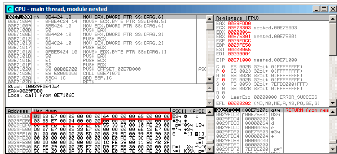
Figure 1.108: OllyDbg: Before printf() execution
