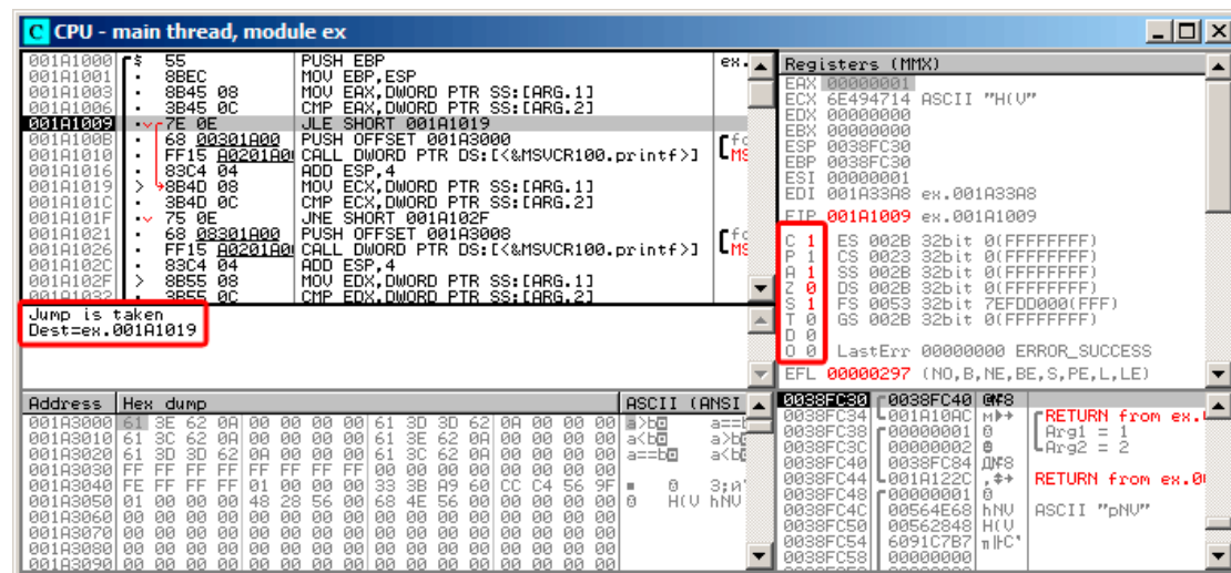
Figure 1.38: OllyDbg: f_signed() : first conditional jump
