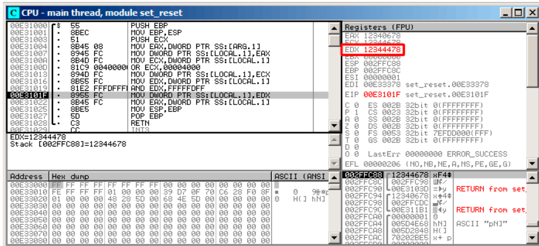
Figure 1.98: OllyDbg: AND executed
