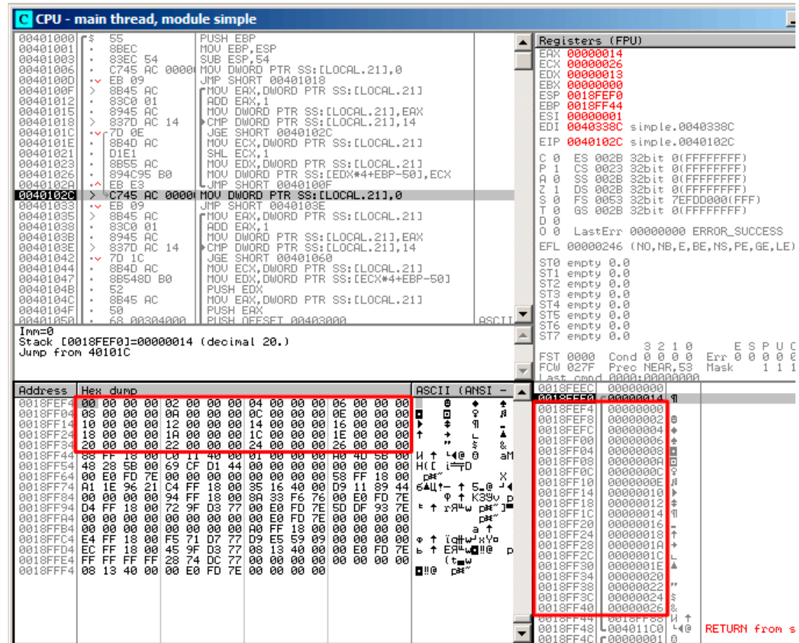
Figure 1.88: OllyDbg: after array filling
