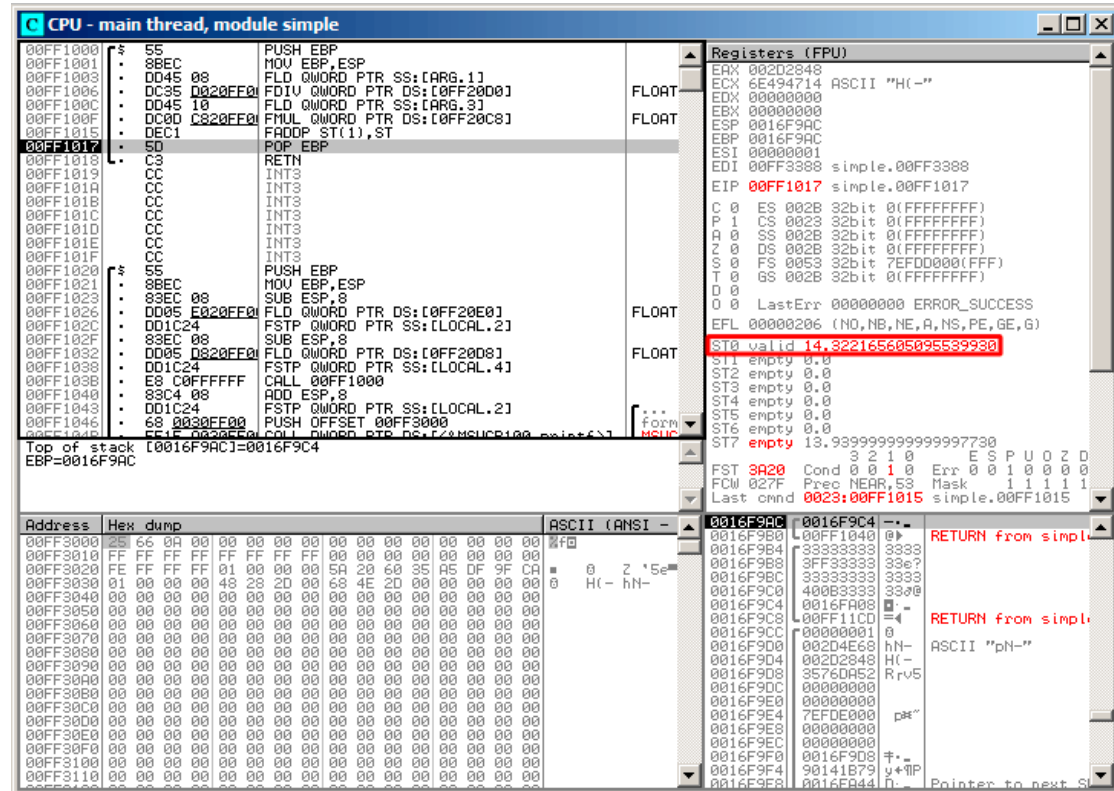
Figure 1.67: OllyDbg: FADDP has been executed
