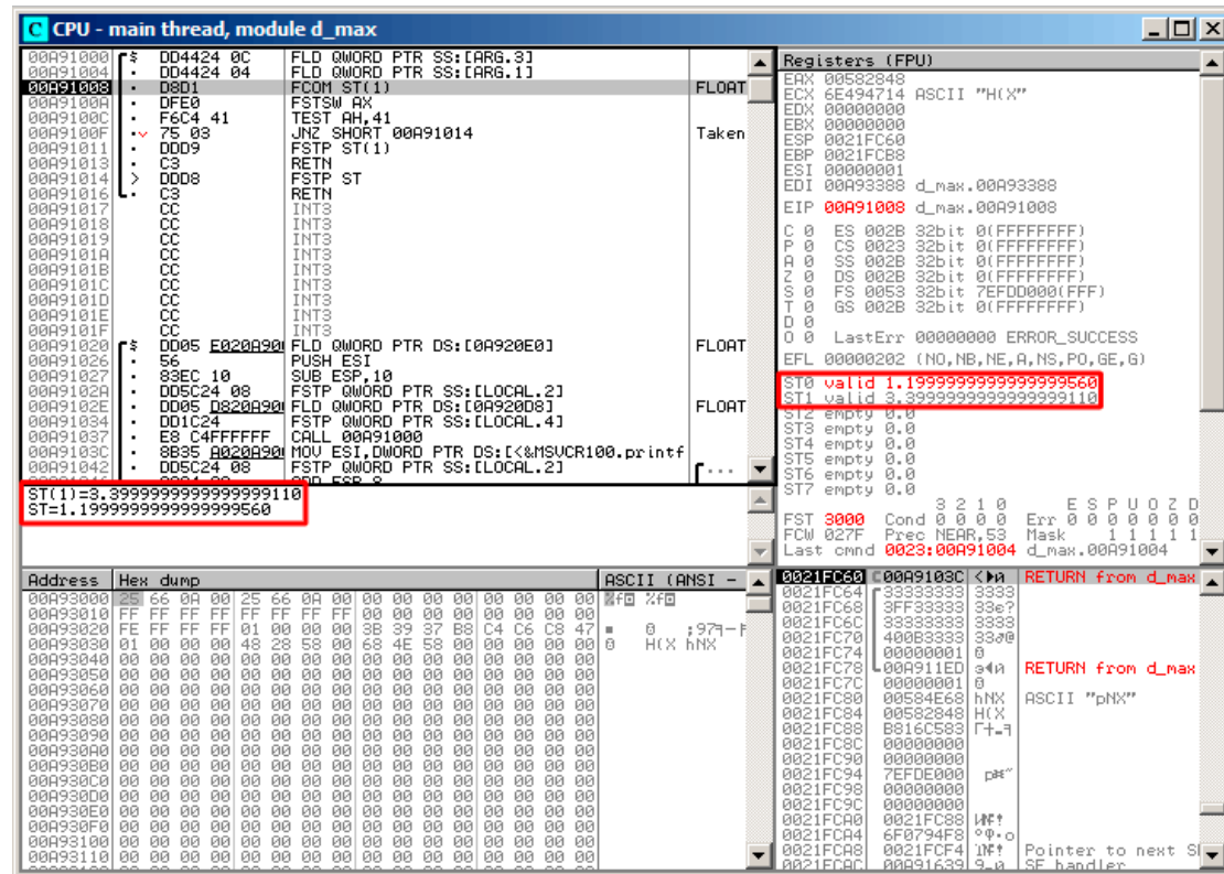
Figure 1.78: OllyDbg: both FLD are executed
