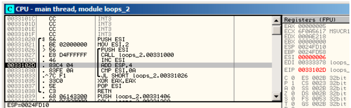
Figure 1.56: OllyDbg: loop body just executed with i = 6
