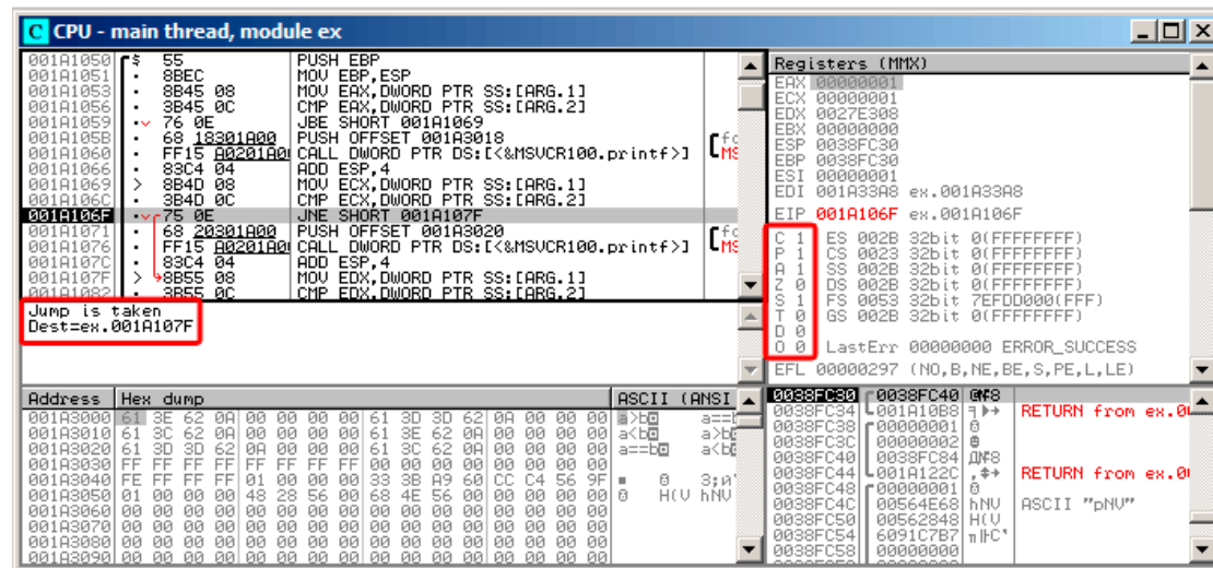
Figure 1.36: OllyDbg: f_unsigned(): second conditional jump
