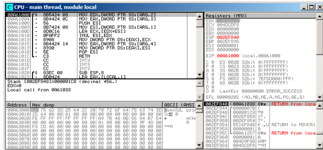
Figure 1.31: OllyDbg: f1() starting
