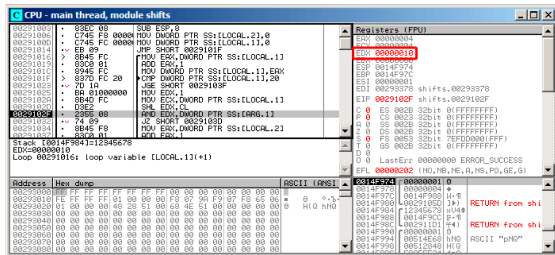
Figure 1.103: OllyDbg: i = 4 , EDX = 1 \ll 4 = 0x10
