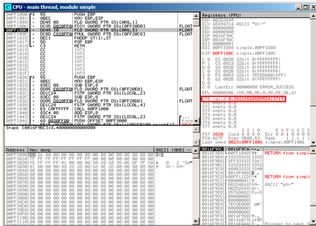
Figure 1.64: OllyDbg: FDIV has been executed
