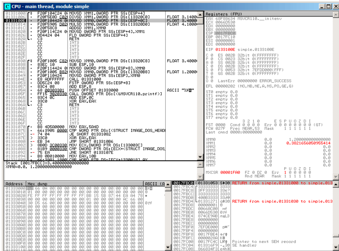
Figure 1.115: OllyDbg: DIVSD calculated quotient and stored it in XMM1
