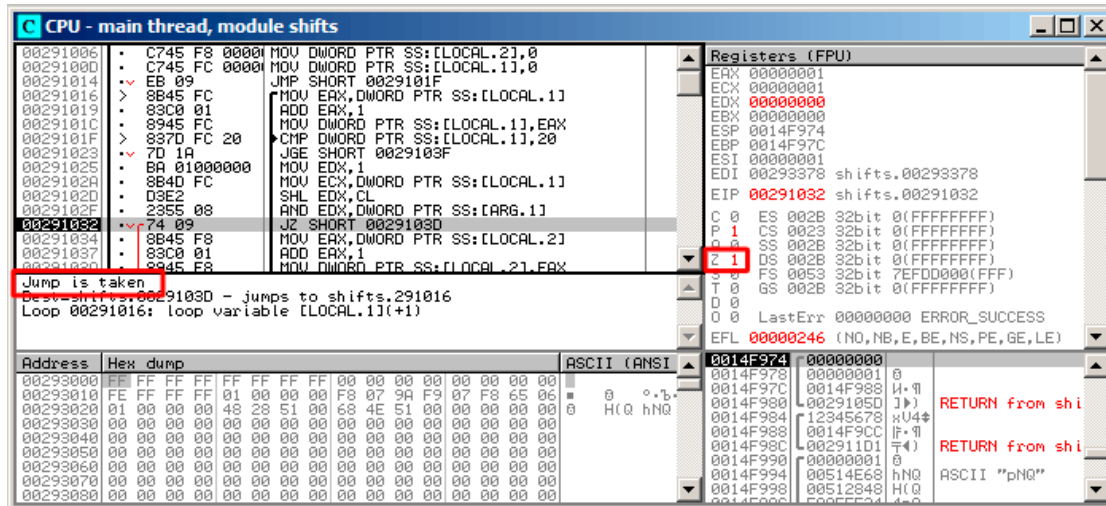
Figure 1.101: OllyDbg: i = 1 , is there that bit in the input value? No. (ZF = 1)
