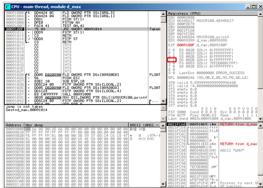
Figure 1.86: OllyDbg: TEST has been executed
