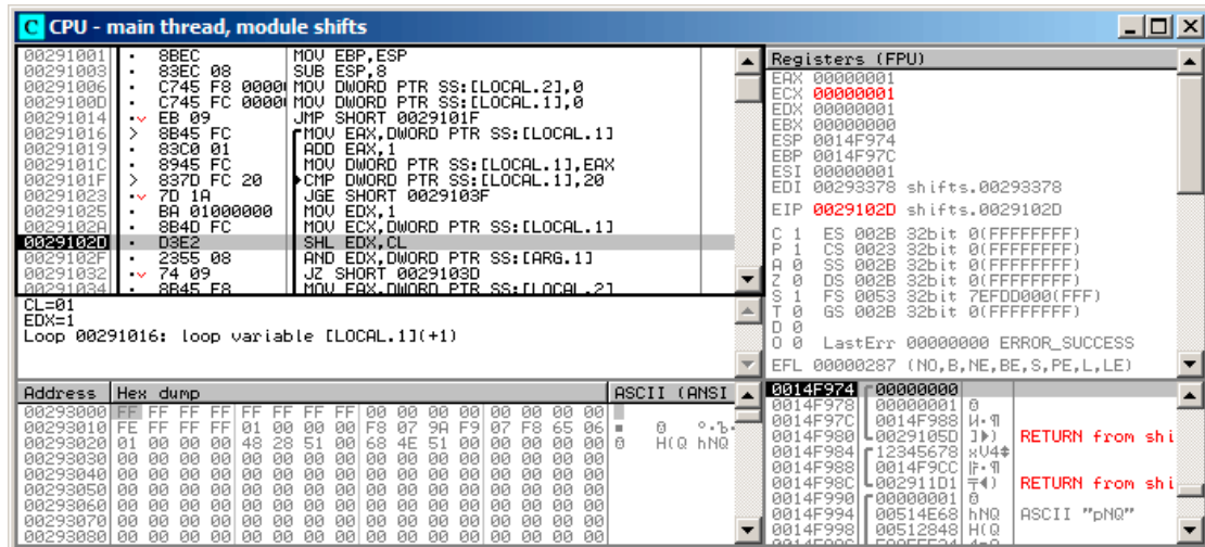
Figure 1.99: OllyDbg: i = 1 , i is loaded into ECX
