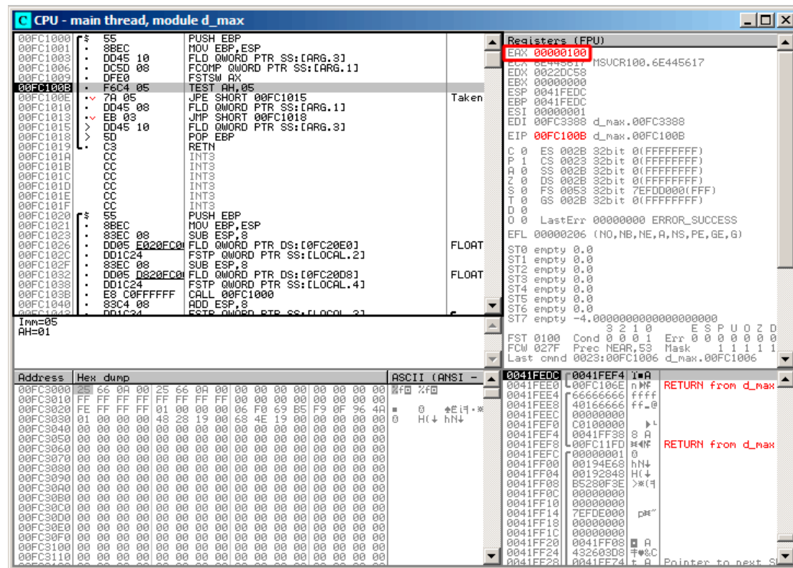
Figure 1.75: OllyDbg: FNSTSW executed
